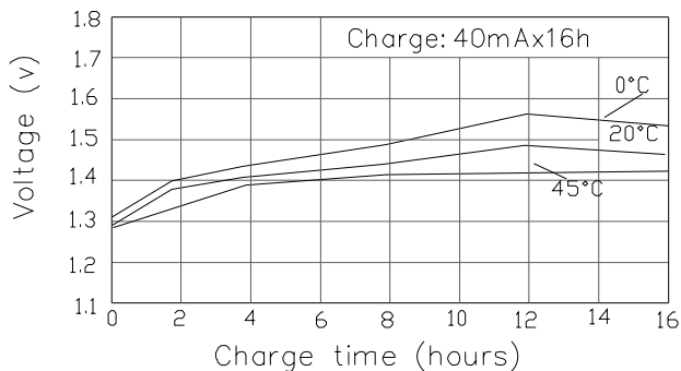
Standard charge
