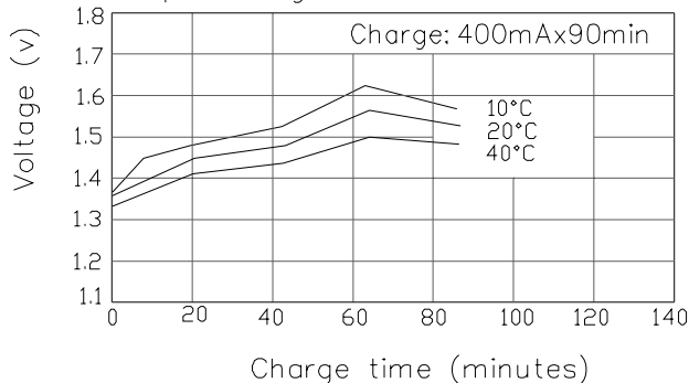
Rapid charge
