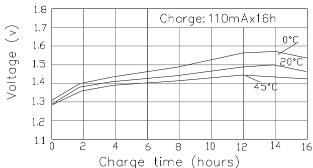
Standard charge
