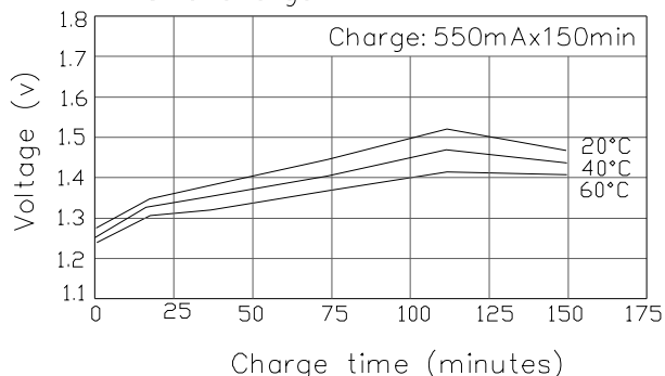
Trickle charge
